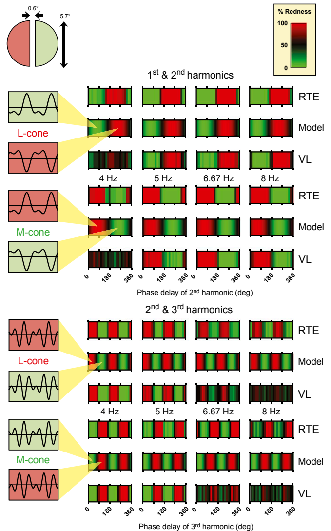
Fig. 3. The illustration in the top left corner shows the stimulus configuration: 5.7° hemifields separated by a 0.6° gap. Data for two observers R.T.E. and V.L. and predictions for two different two-component waveforms are shown in four columns, with each column corresponding to a different fundamental frequency. Upper shows results for a fundamental and second harmonic in the amplitude ratio 1.0:0.5. Rows 1–3 in Upper are for L cone-isolating stimuli, and rows 4–6 in Upper are for M cone-isolating stimuli. The colors in the panels correspond to the scale labeled as “percent redness”. In the data panels, the colors indicate the percentage of times that each phase combination was indicated by the observer as appearing redder than its inverse. Black here corresponds to 50%, which we take to mean no reliable color shift between the two waveforms (i.e., one waveform and its inverse were equally likely to be chosen as redder). The colors in the model panels indicate the predicted color shift given by our model. The predictions have been scaled so that the largest shift toward red corresponds to a score of 100 and the largest shift toward green corresponds to 0, with 50 (shown as black) meaning no color shift. Each panel in Upper has the phase delay (in degrees) of the second harmonic on the abscissa. Lower shows results and model predictions for second and third harmonics of equal amplitude (the optimal modulation ratio of these harmonics according to the model) in the same format as Upper . Each panel has the phase delay (in degrees) of the third harmonic on the abscissa. Measurements were made at 15° intervals; the model's predictions are given at 1° intervals. The waveforms in the Left Insets illustrate the optimal waveforms for producing red and color shifts according to the model, which have the harmonic phase delays indicated by the tips of the yellow cones.
